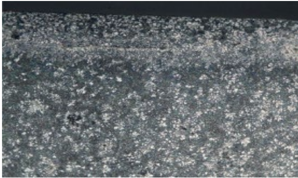
The surface of the laser-cleaned light alloy part forms a microcrystalline respectively amorphous boundary layer, free of contamination and with decreased electrochemical potential
